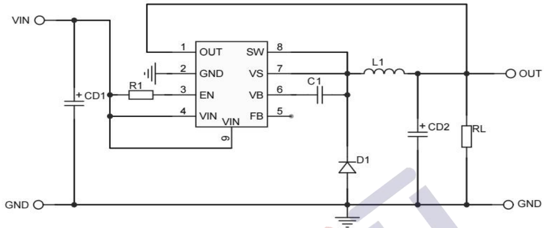
APP1: V_{OUT}<10V
